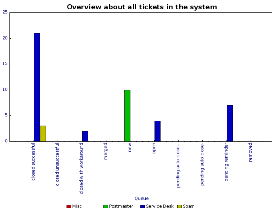
Figure 10.6. ticket-graphic-overview
