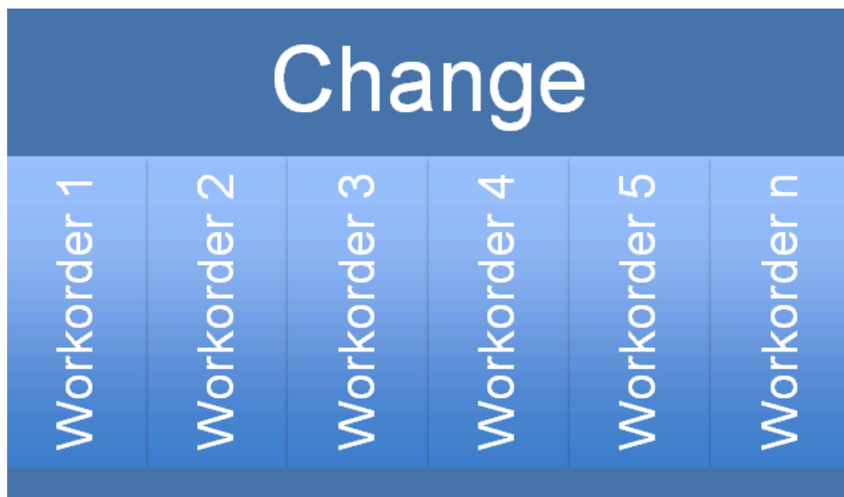
Figure 8.1. change-workorder-schema
