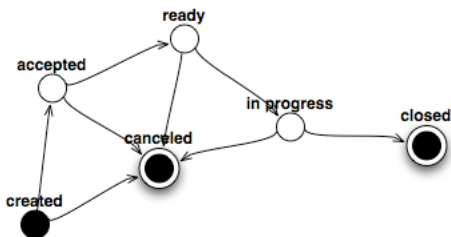
Figure 8.11. change-workorder-state-machine
