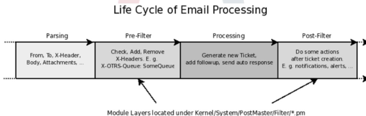
Figure 3.6. Email Processing Flow
