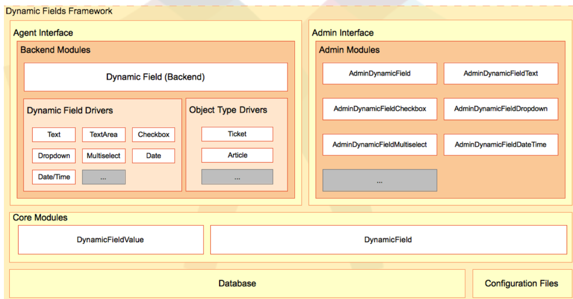
Figure 3.4. Dynamic Fields Architecture
