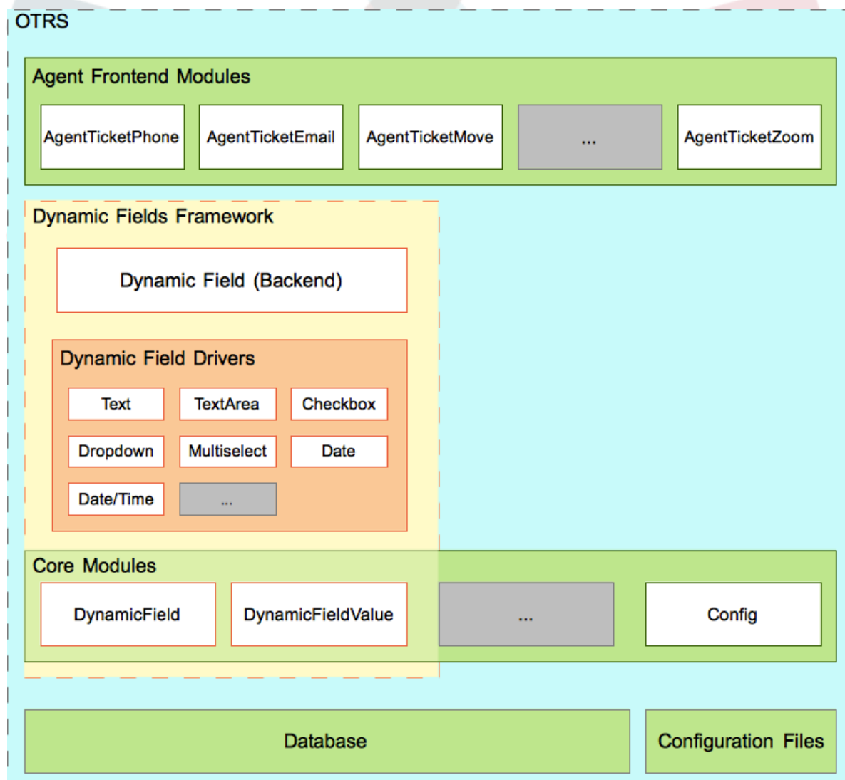
Figure 3.5. Dynamic Field Interaction
