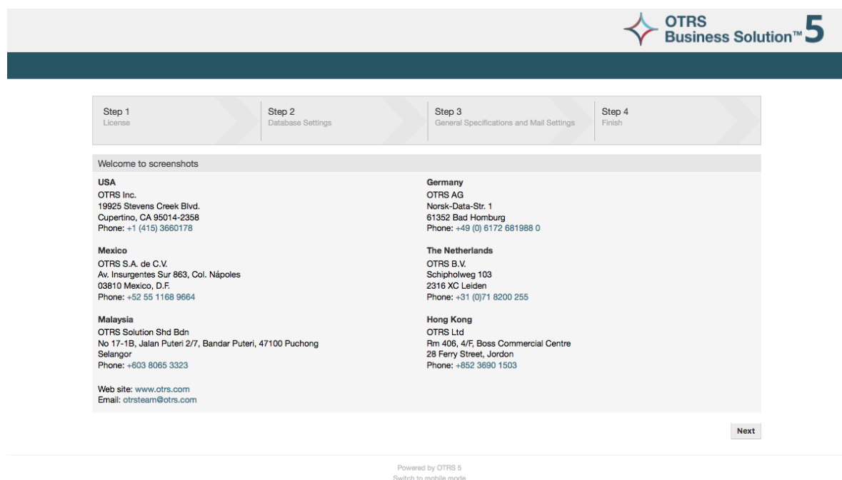
Figure 2.1. Welcome screen
