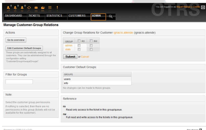
Figure: Change Group relations for a Customer.
